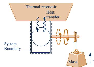
Fig. 5.4 System undergoing a cycle while exchanging energy by heat transfer with a single thermal reservoir.
