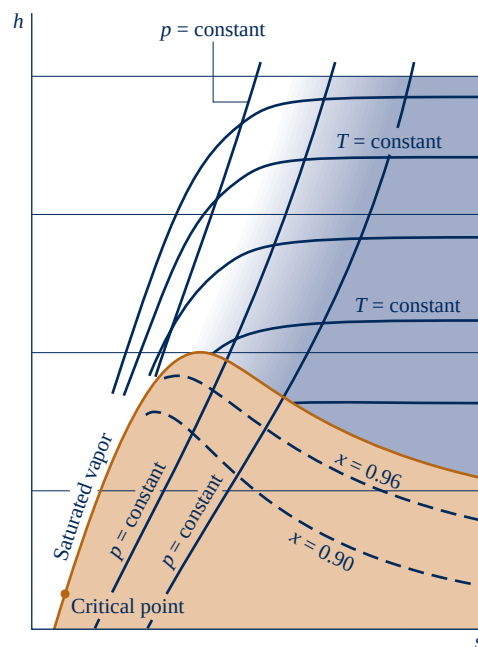
Fig. 6.3 Enthalpy–entropy diagram.
