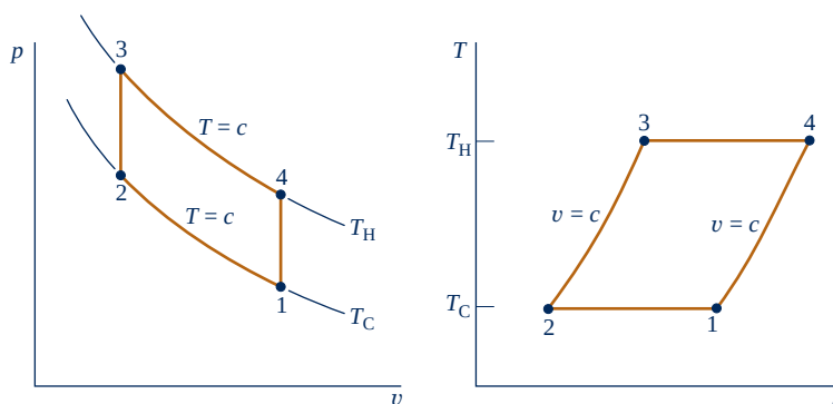
Fig. 9.21 p - v and T - s diagrams of the Stirling cycle.
