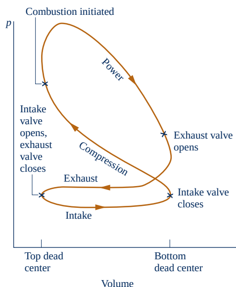
(9.1) Fig. 9.2 Pressure–volume diagram for a reciprocating internal combustion engine.
