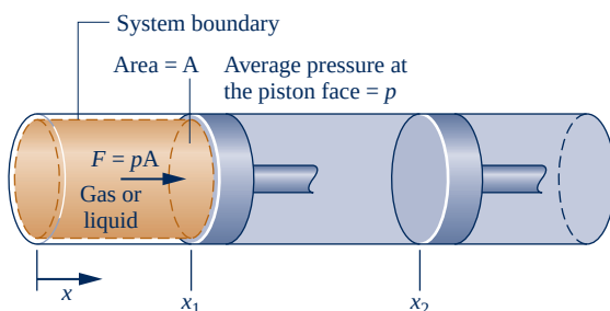
Fig. 2.4 Expansion or compression of a gas or liquid.
