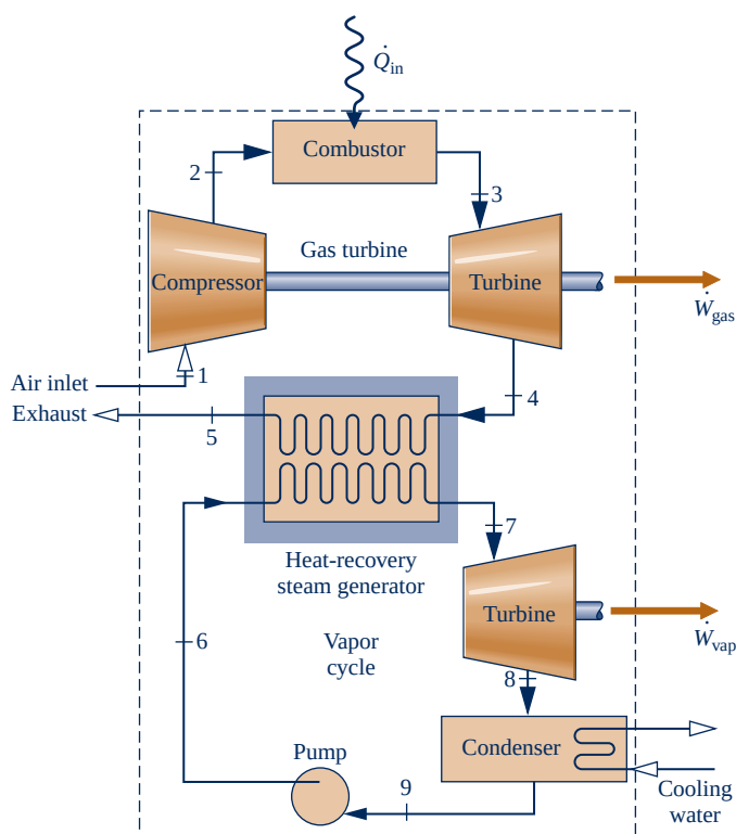
Fig. 9.22 Combined gas turbine–vapor power plant.
