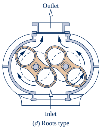
Fig. 4.11 Compressor types.
