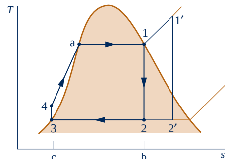
Fig. 8.3 Temperature–entropy diagram of the ideal Rankine cycle.
