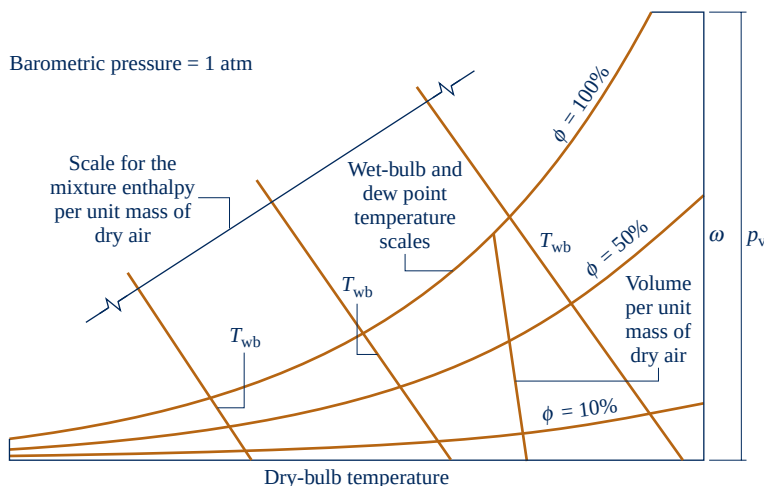
Fig. 12.9 Psychrometric chart.
