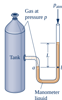
Fig. 1.7 Manometer.
