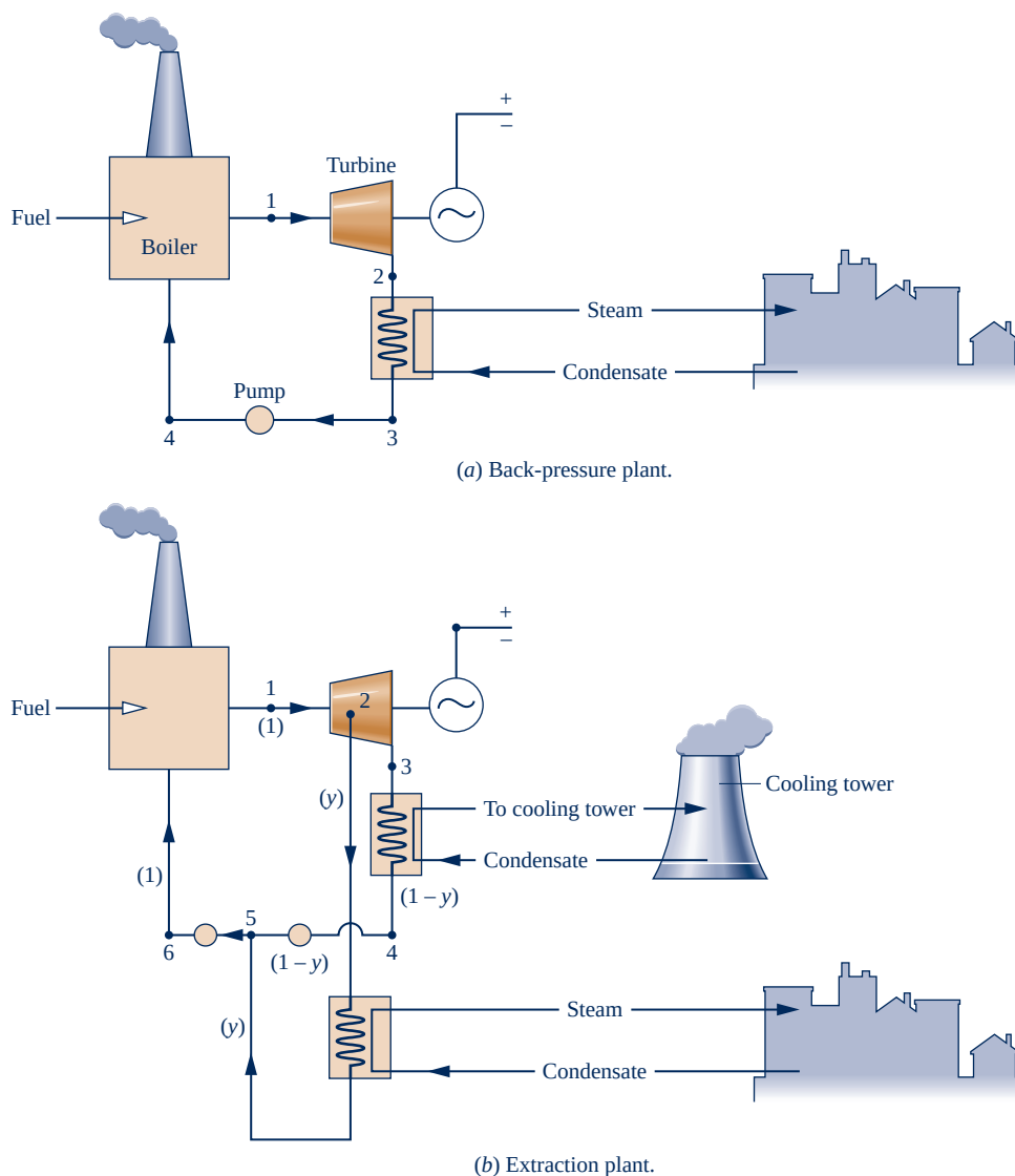
Fig. 8.14 Vapor cycle district heating plants.
