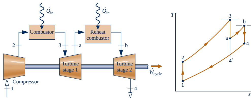
Fig. 9.16 Ideal gas turbine with reheat.
