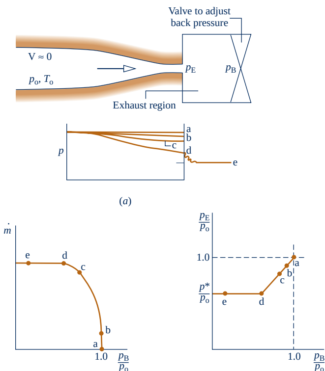
Fig. 9.31 Effect of back pressure on the operation of a converging nozzle.
