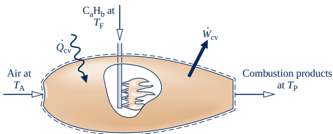
Fig. 13.2 Reactor at steady state.
