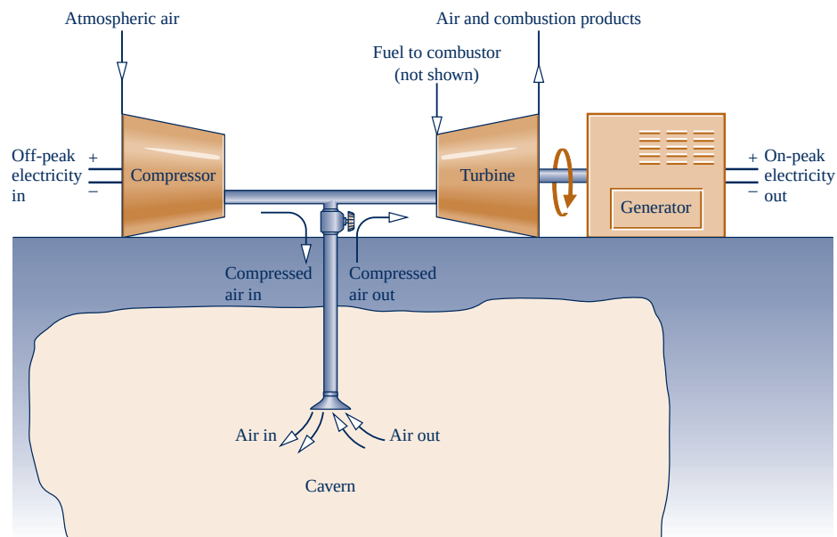
Fig. 4.12 Compressed-air storage.
