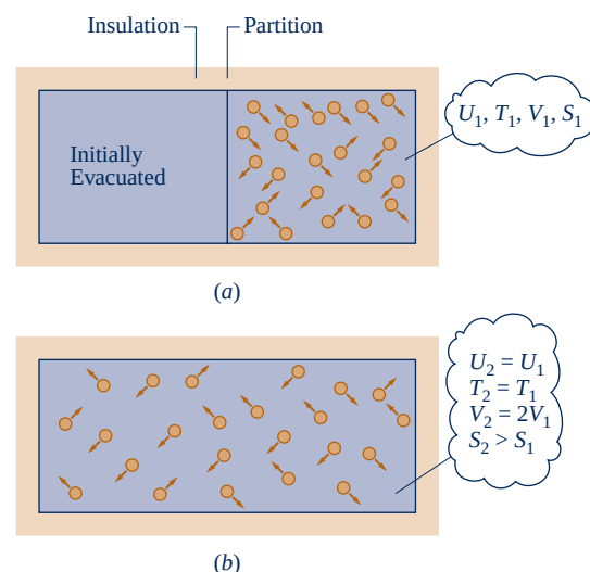
Fig. 6.7 N molecules a box.
