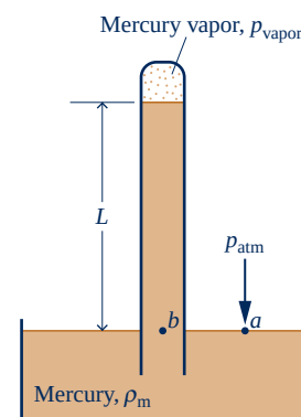
Fig. 1.8 Barometer.
