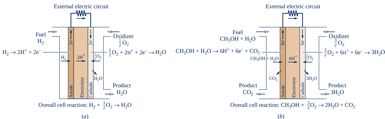
Fig. 13.3 Proton exchange membrane fuel cell. (a) Hydrogen fueled. (b) Humidified-methanol fueled.
