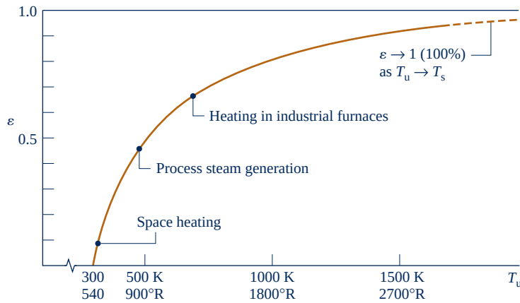
Fig. 7.8 Effect of use temperature T_u on the exergetic efficiency \varepsilon ( T_s = 2200 \text{ K} , \eta = 100\% ).
