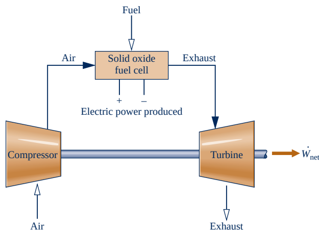
Fig. 13.5 Solid oxide fuel cell–microturbine hybrid.
