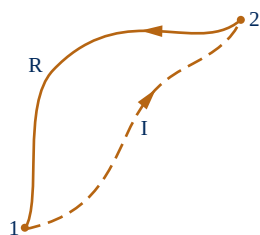
Fig. 6.6 Cycle used to develop the entropy balance.
