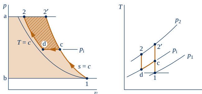
Fig. 9.18 Two-stage compression with intercooling.
